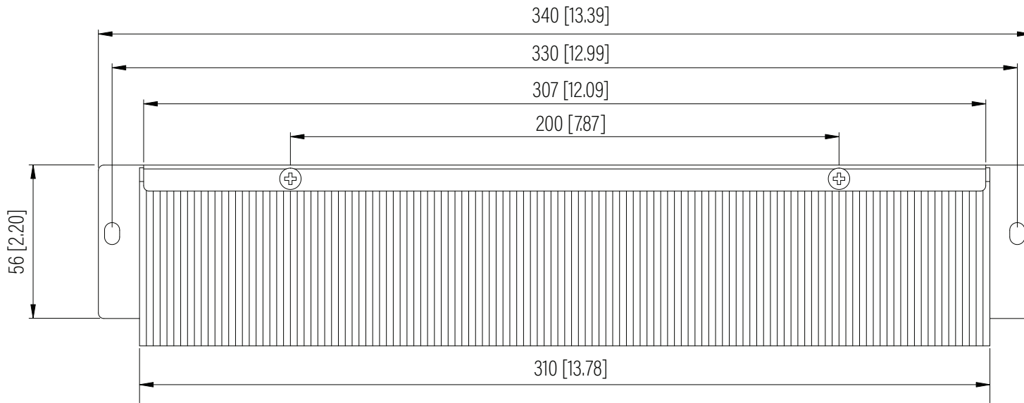
Rear View
